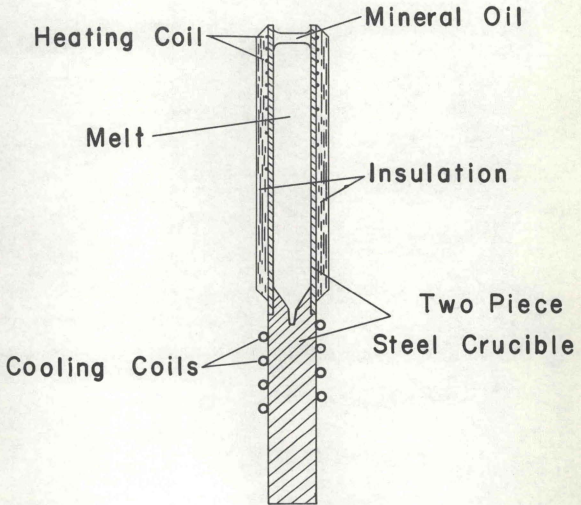
Figure 1. Crucible for growing sodium crystals.
